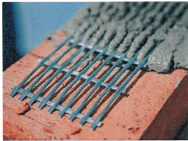
Figure 2 – Typical installation in a horizontal masonry bed joint
